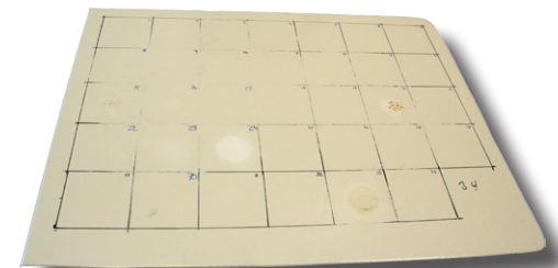
Tested panel (bottom) and close-up (top) on tests for sulfuric acid 33%, 77% and 96%
