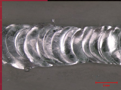
Macroscopic View of Titanium Groove Weld
